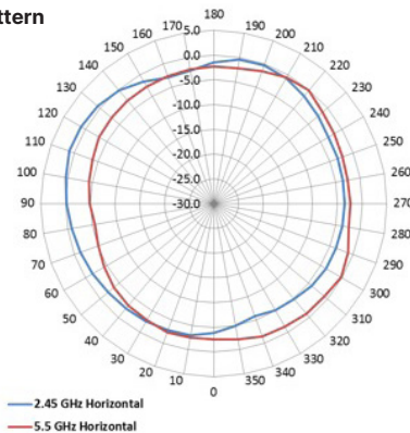
E-Plane Pattern
